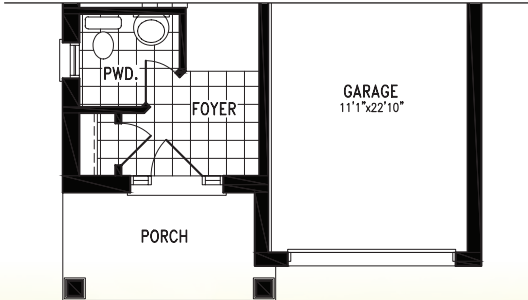
Partial Ground Floor Plan 'C'
