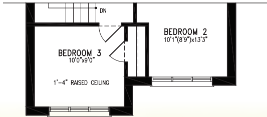
Partial Second Floor Plan 'C'
