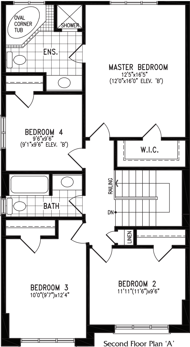
Second Floor Plan 'A'
