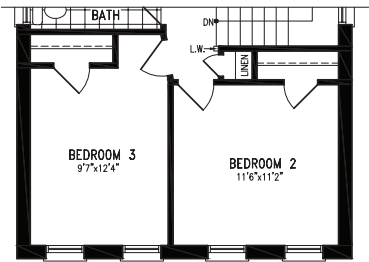
Partial Second Floor Plan 'C'
