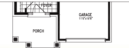
Partial Ground Floor Plan 'B'
