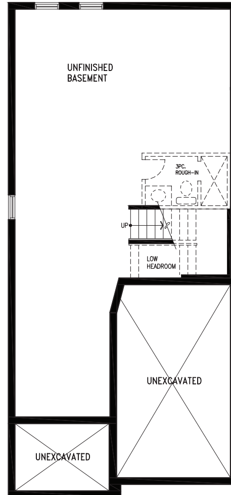
Basement Floor Plan 'A'
