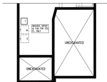
Partial Basement Floor Plan 'C'
