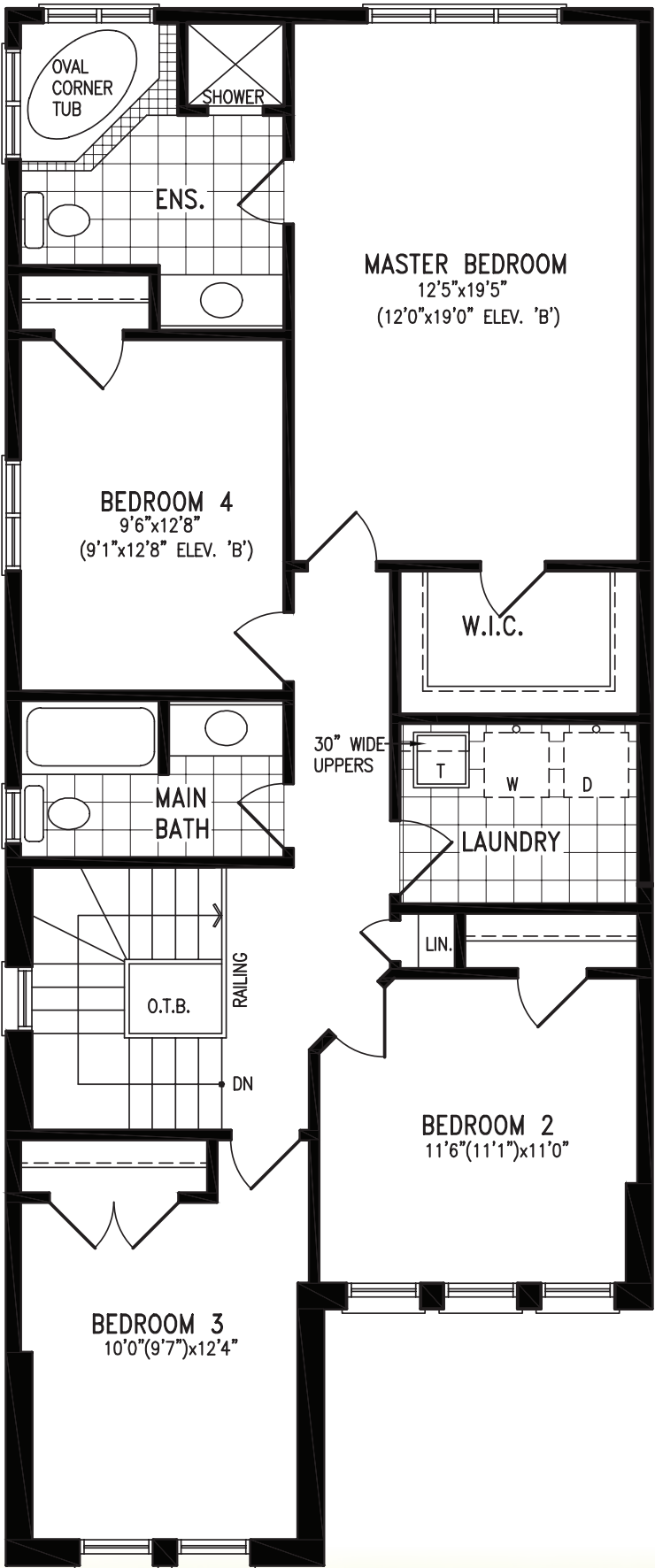
Second Floor Plan 'A'
