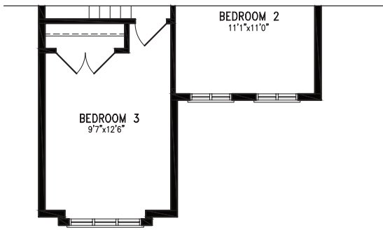
Partial Second Floor Plan 'B'
